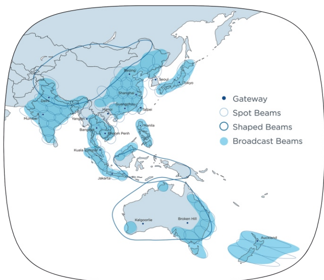
Thaicom-4 Footprint for Thailand Coverage
